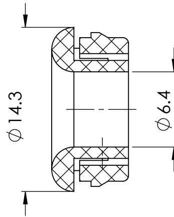
SECTION Y-Y
