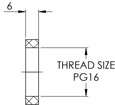
SECTION Y-Y
