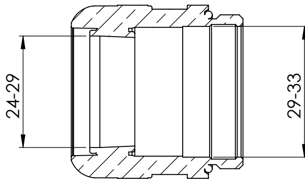
SECTION X-X
