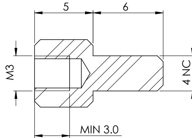
SECTION Y-Y
