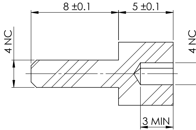
SECTION Y-Y
