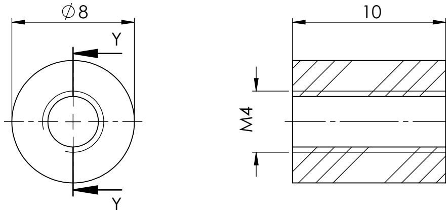
SECTION Y-Y
