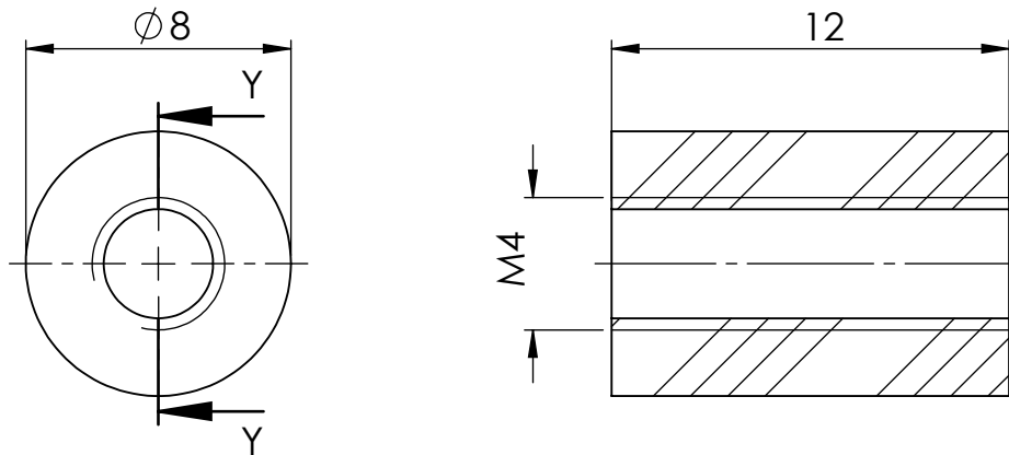
SECTION Y-Y
