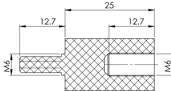
SECTION Y-Y
