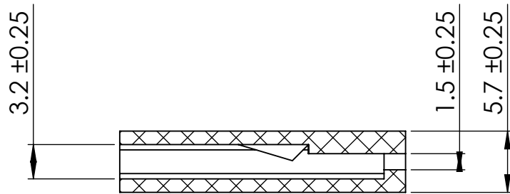
SECTION Y-Y
