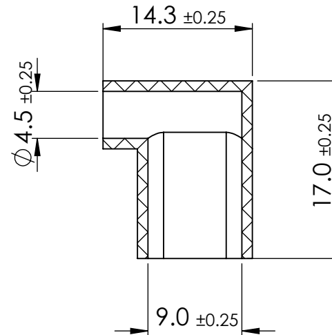
SECTION Y-Y
