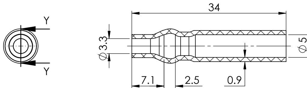
SECTION Y-Y
