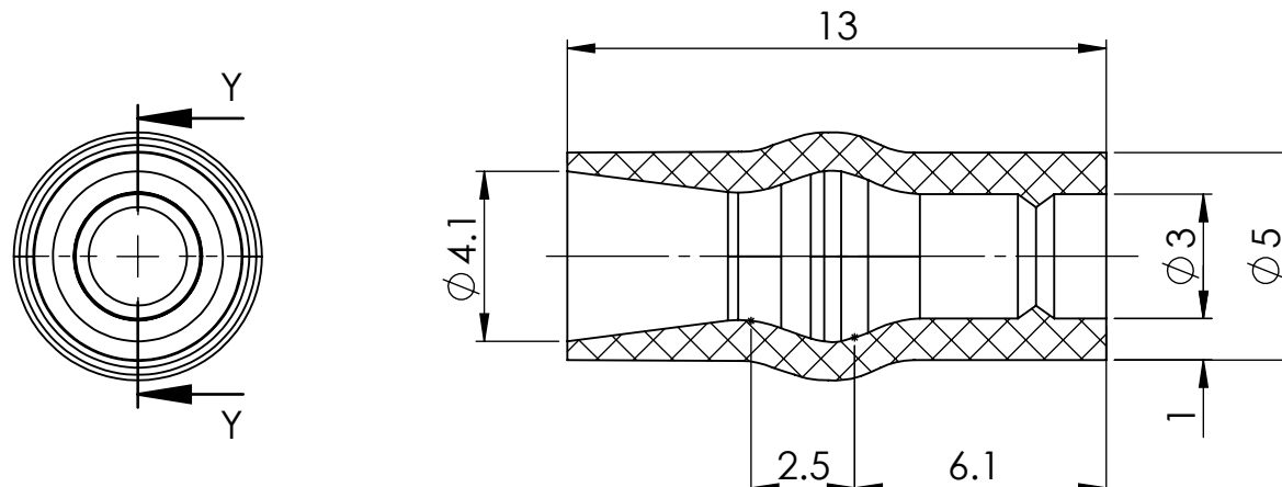
SECTION Y-Y
