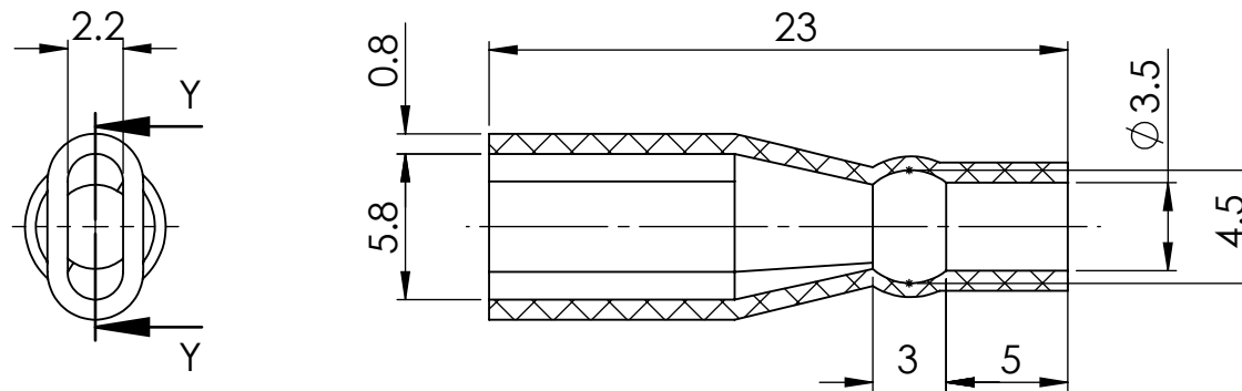
SECTION Y-Y
