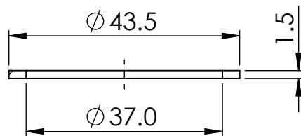
SECTION X-X
