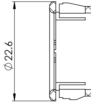
SECTION Y-Y
