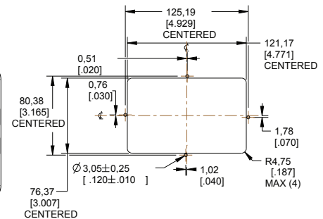
PANEL CUTOUT AND MOUNTING INFORMATION ALL DIMENSIONS ARE \pm 0.50\text{mm} (PANEL THICKNESS TO BE 2.5 \pm 1.0\text{mm} )
