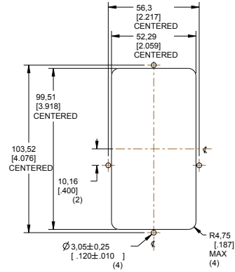
PANEL CUTOUT AND MOUNTING INFORMATION ALL DIMENSIONS ARE \pm 0.50\text{mm} (PANEL THICKNESS TO BE 2.5 \pm 1.0\text{mm} )
