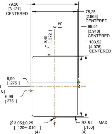
PANEL CUTOUT AND MOUNTING INFORMATION ALL DIMENSIONS ARE \pm 0.50\text{mm} (PANEL THICKNESS TO BE 2.5 \pm 1.0\text{mm} )
