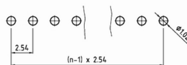
PCB Layouts
