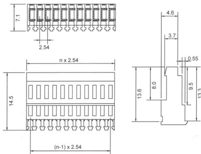
Housing
