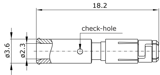
Main Dimension contact socket
