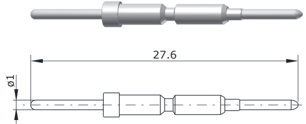
Main Dimensions contact pin
