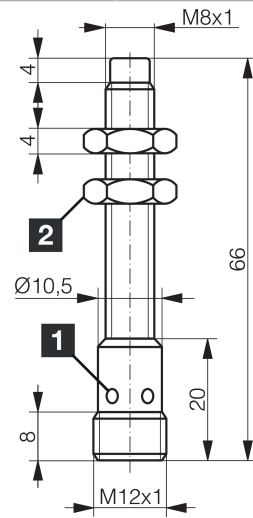
1) LED 4 x 90° (gelb) / LED 4 x 90° (yellow) / LED 4 x 90° (jaune) 2) Schlüsselweite 13 mm / Width over flats 13 mm / Ouverture de clé 13 mm mm
