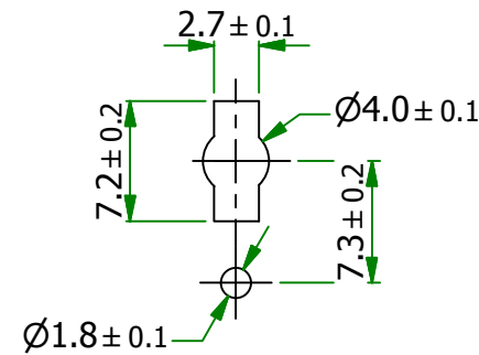
BOTTOM FIXING HOLE DETAILS
